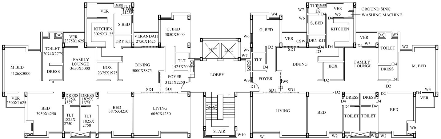
8 STORIED B -TYPE QTR TYPICAL FLOOR PLAN
