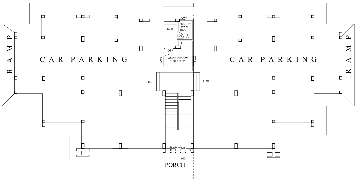
'C' TYPE QUARTER GROUND FLOOR PLAN
