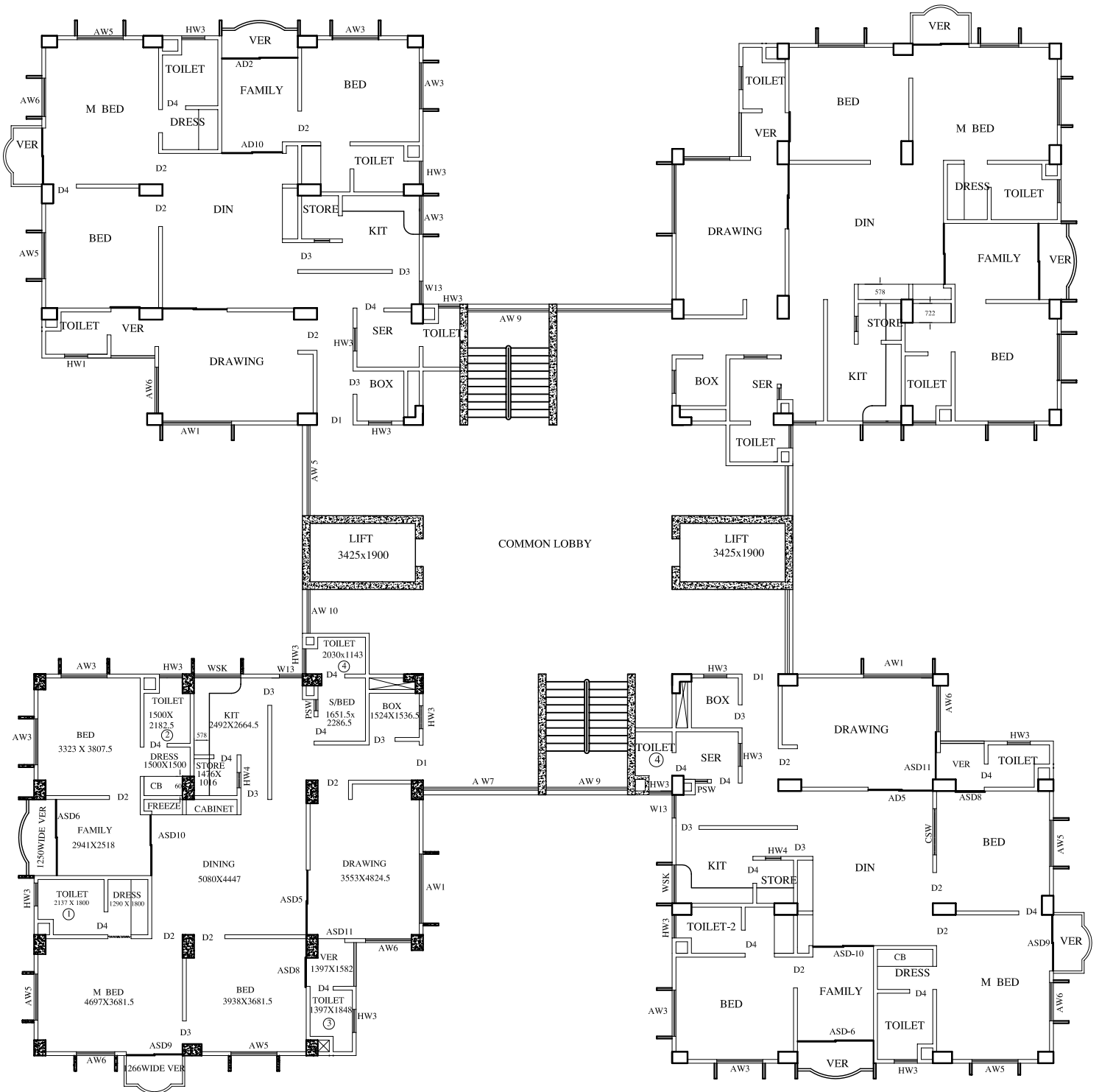
14-STORIED 'D' TYPE OFFICERS QTR TYPICAL FLOORPLAN
