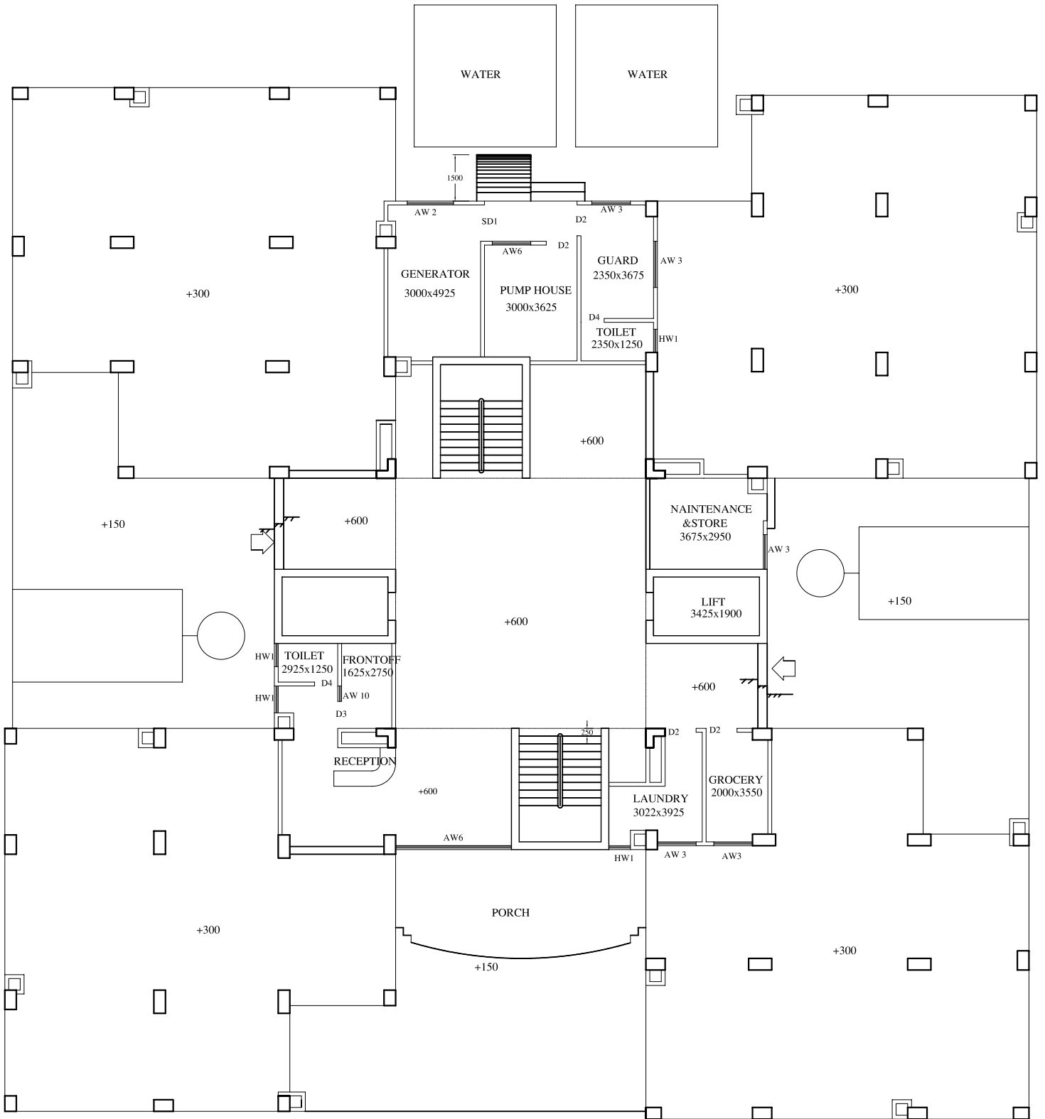
14-STORIED 'D' TYPE OFFICERS QTR GROUND FLOOR PLAN
