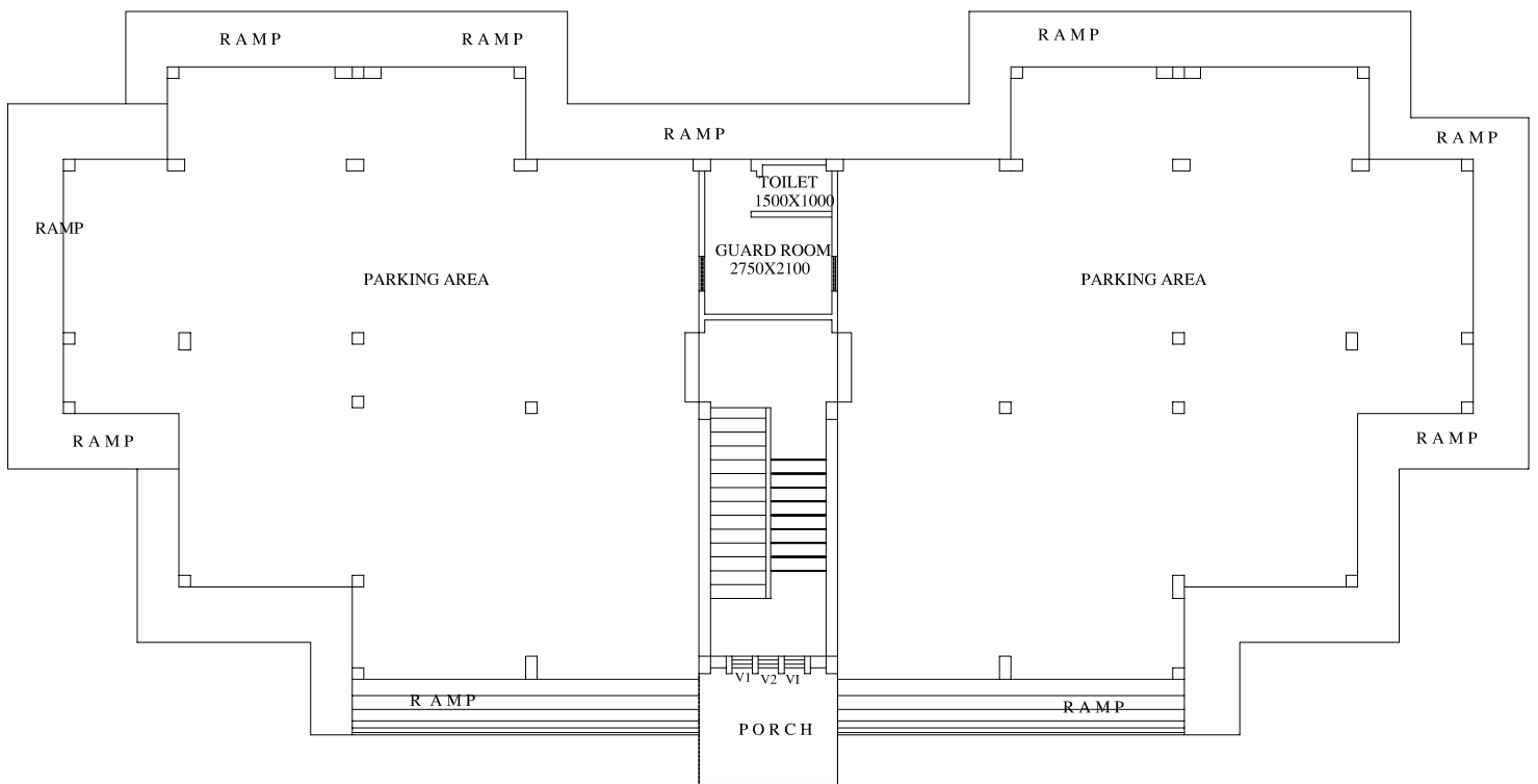
D TYPE QTR GROUND FLOOR PLAN
