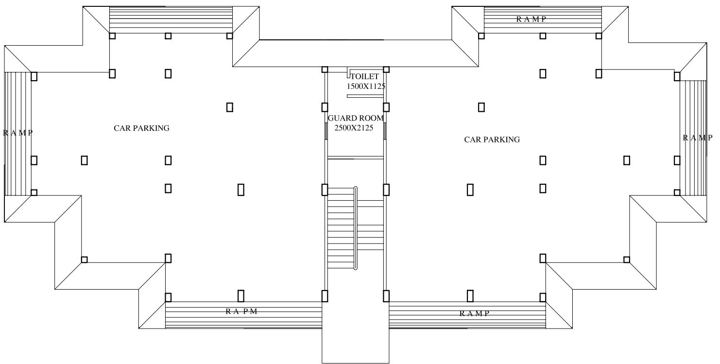
'E' TYPE QTR GROUND FLOOR PLAN
