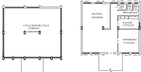
1ST & TYPICAL FLOOR PLAN
