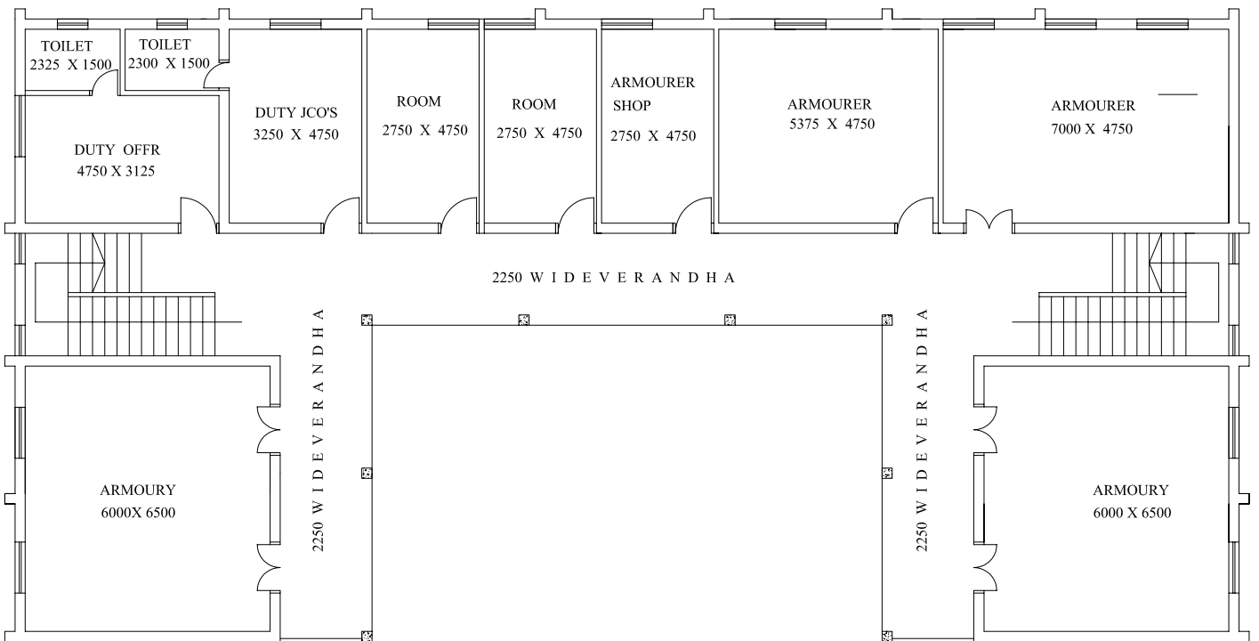
QUARTER GUARD (TYPE-B) FIRST FLOOR PLAN
