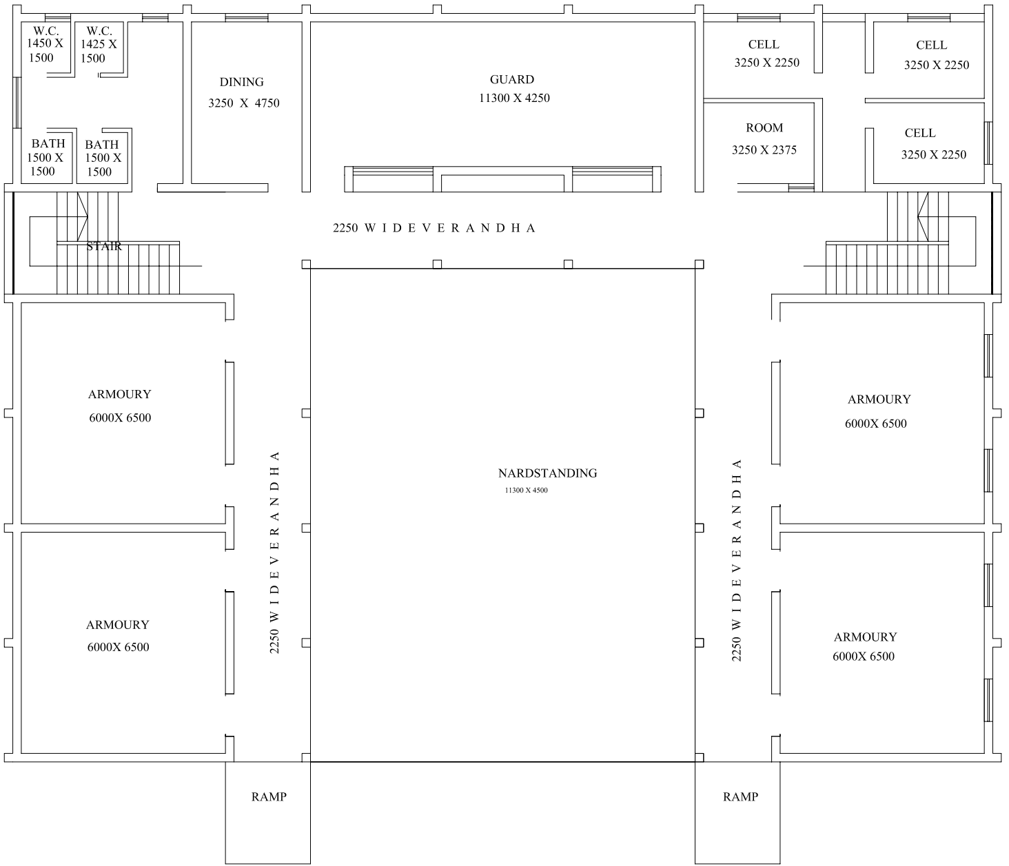
QUARTER GUARD (TYPE-A) GROUND FLOOR PLAN
