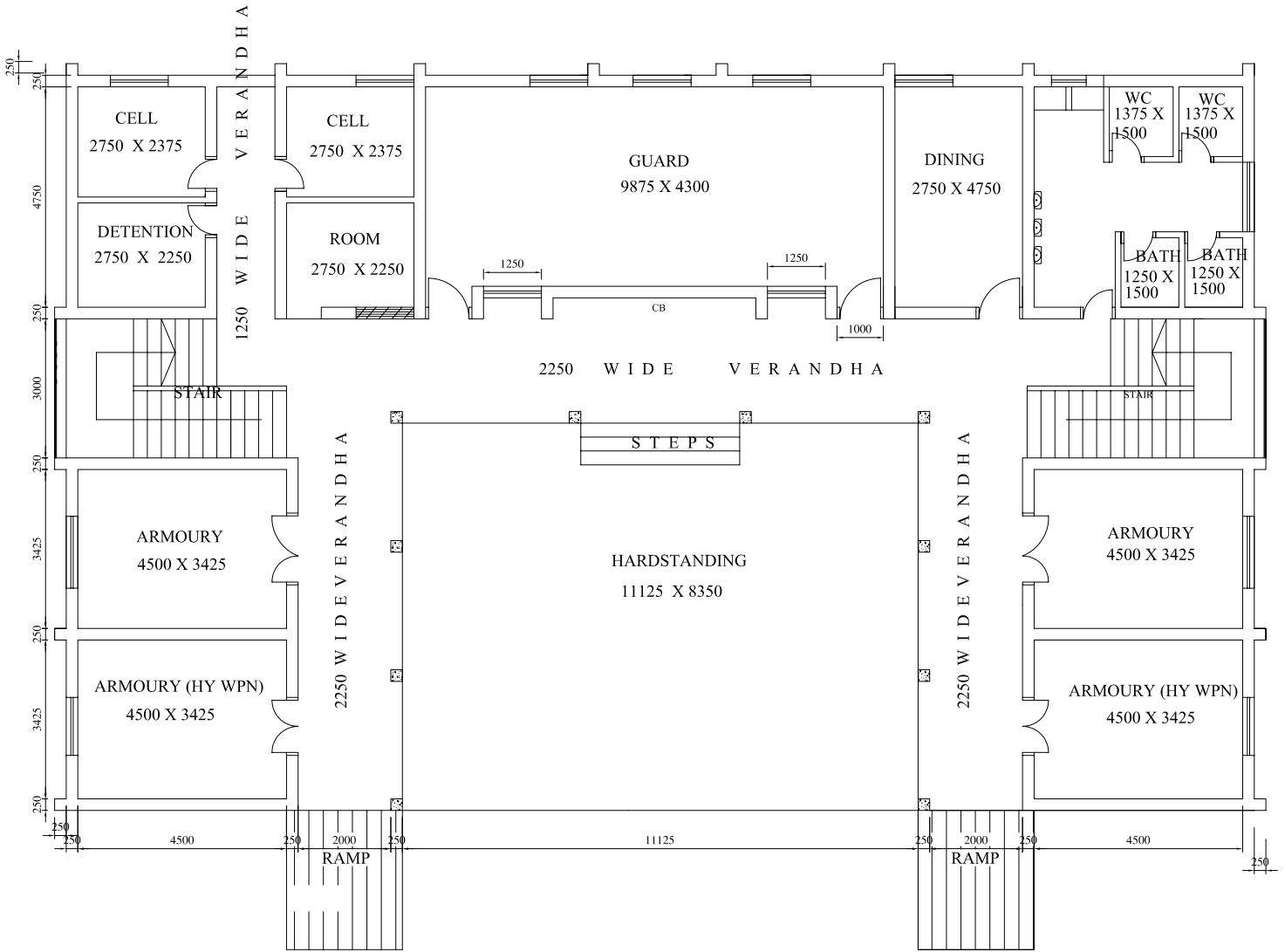
QUARTER GUARD (TYPE- C) GROUND FLOOR PLAN
