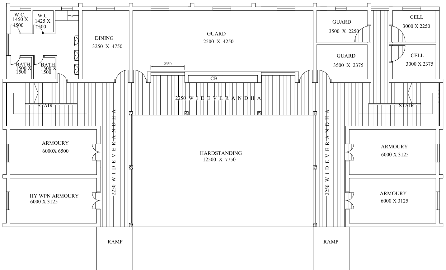
QUARTER GUARD (TYPE-B) GROUND FLOOR PLAN
