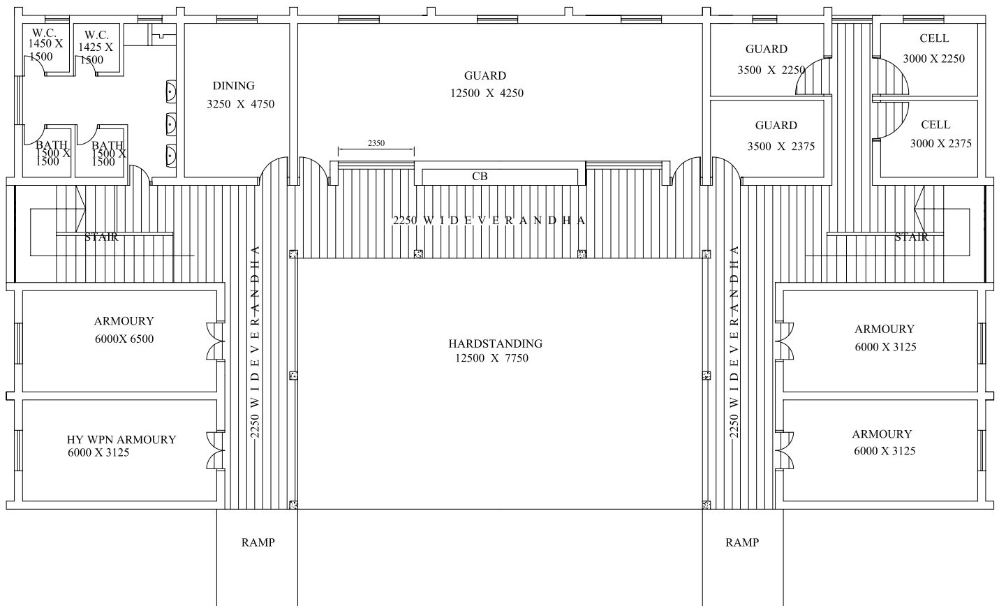
QUARTER GUARD (TYPE-B) GROUND FLOOR PLAN
