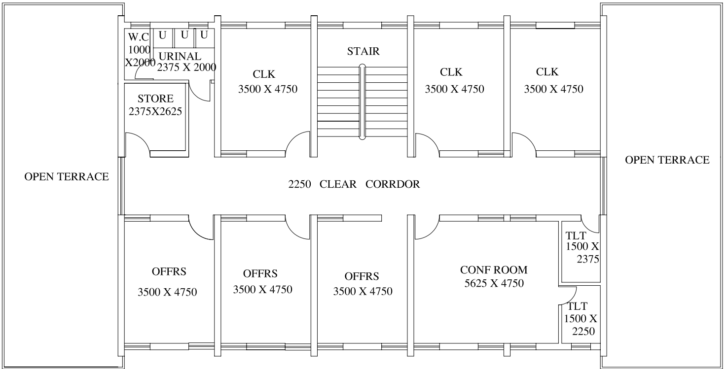
REGT & COY OFFICE (TYPE- C) FIRST FLOOR PLAN
