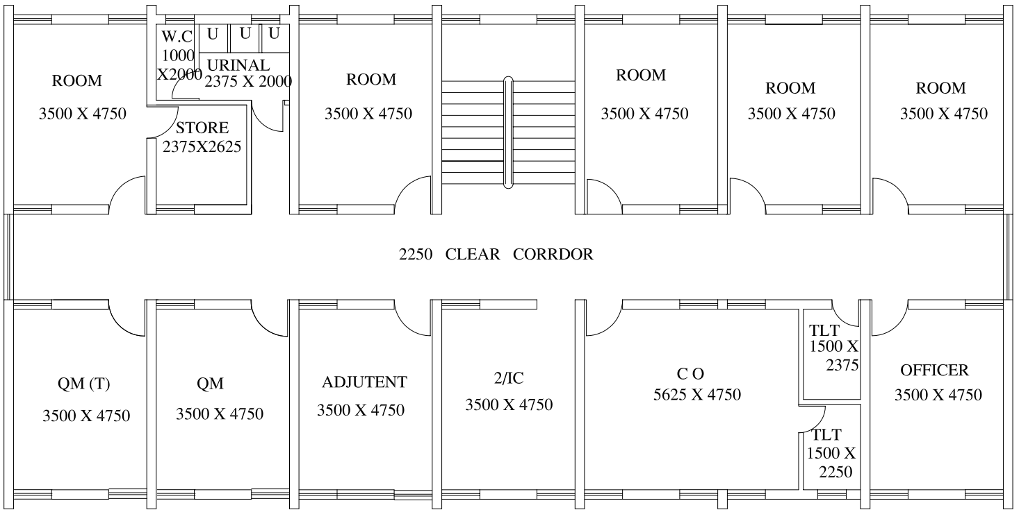
REGT & COY OFFICE (TYPE- B) FIRST FLOOR PLAN
