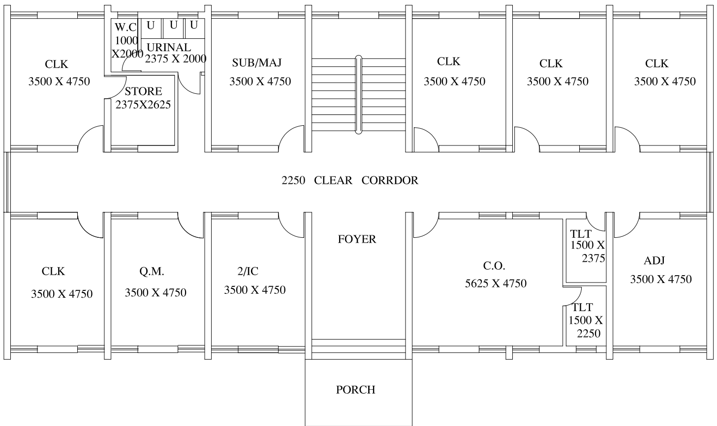
REGT & COY OFFICE (TYPE- C) GROUND FLOOR PLAN
