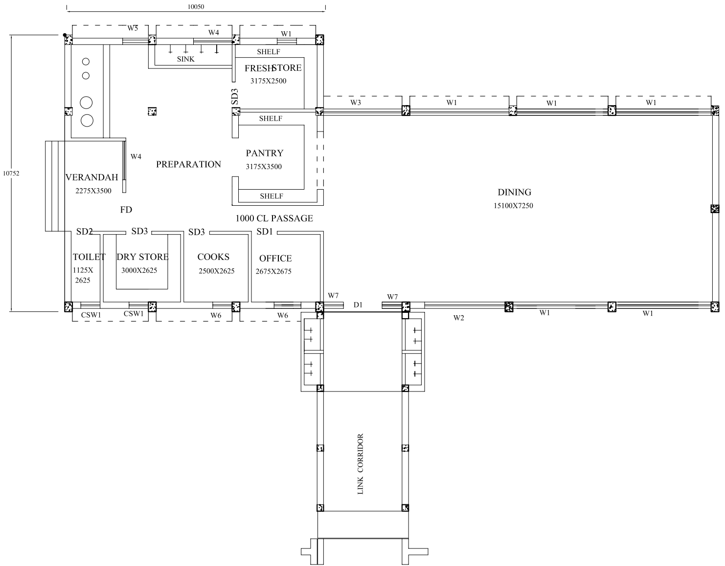
COOK HOUSE & DINING HALL GROUND FLOOR PLAN
