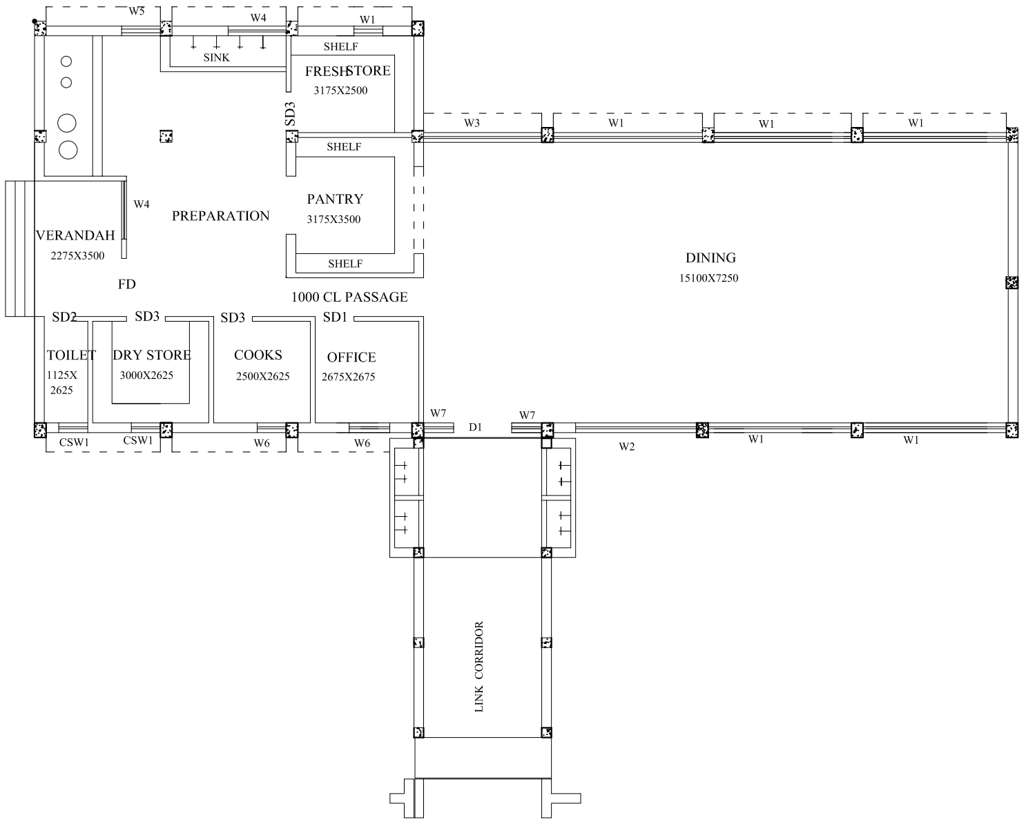
COOK HOUSE & DINING HALL FIRST FLOOR PLAN
