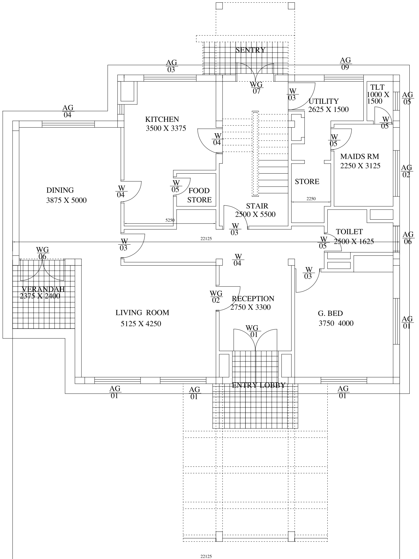
'B' TYPE BUNGLOW GROUND FLOOR PLAN
